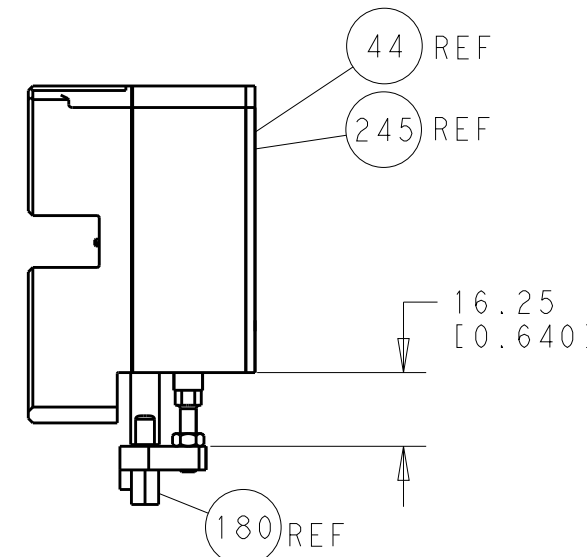
HOLDDOWN SET-UP
