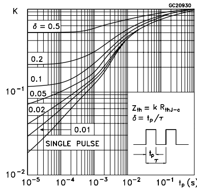
Figure 31. Thermal impedance for diode
