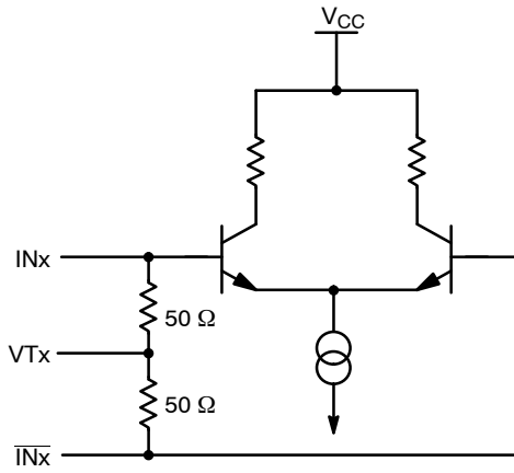
Figure 6. Input Structure
