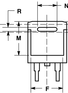
VIEW W-W 2
