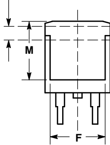
VIEW W-W 1
