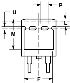
VIEW W-W 3
