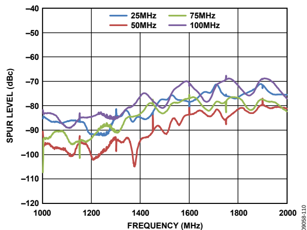
Figure 10. PFD and Reference Spur Levels vs. Frequency at VCO Output, REF_{IN} = 100 MHz, PFD = 25 MHz
