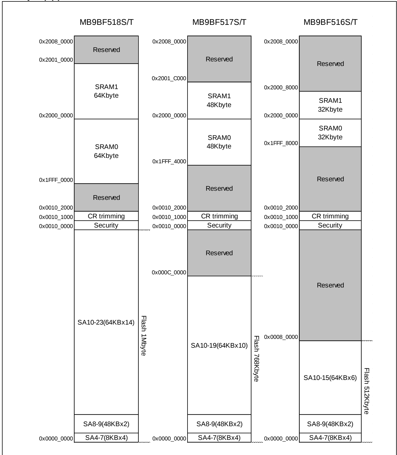
Memory Map (2)
