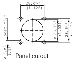
Panel cutout
