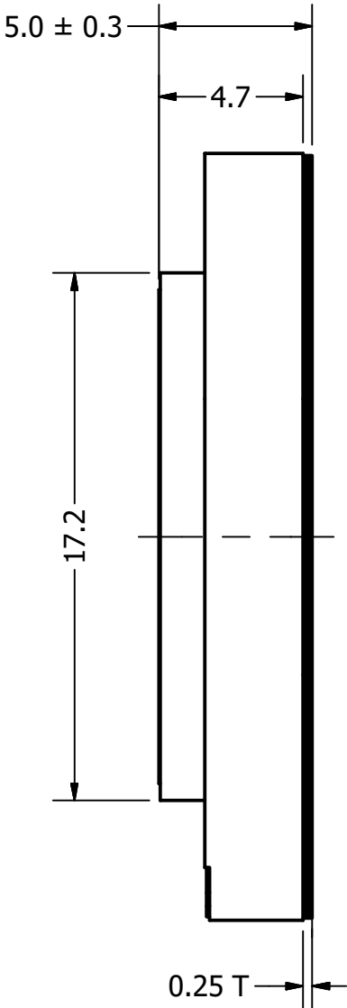
Side View
