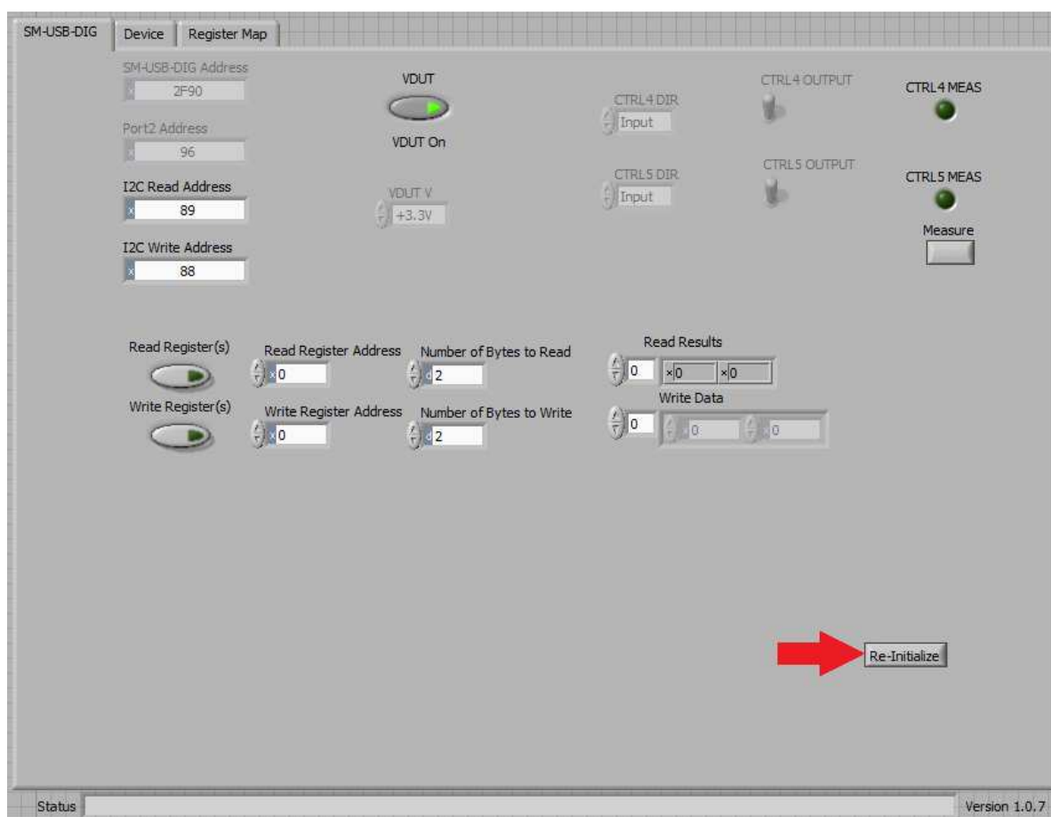
Figure 18. Re-Initialize Button
