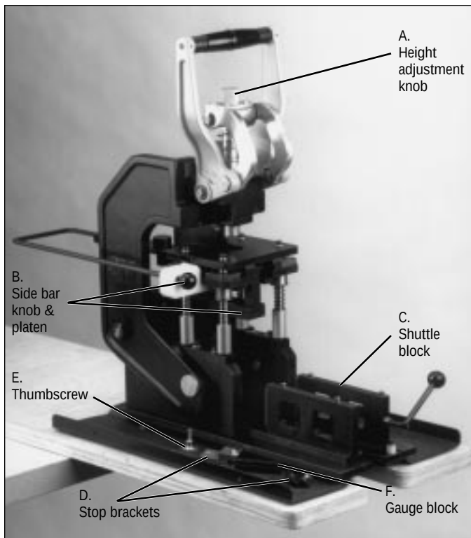
Figure 4. 10960-2000 Hand Press
