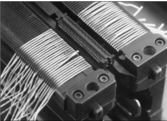
Figure 10. Cut wires
