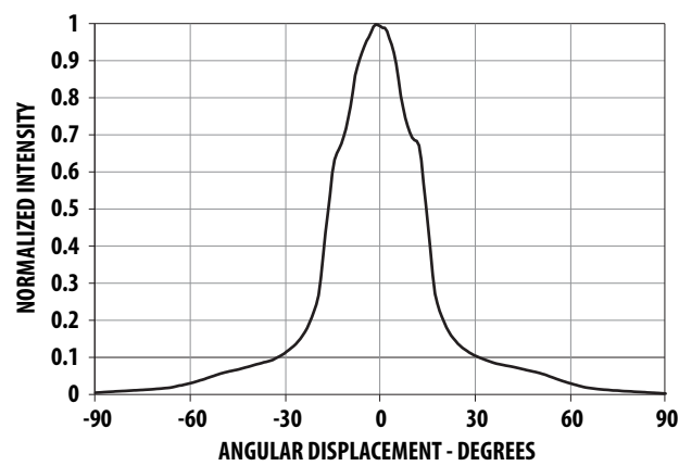
Figure 9: Representative Radiation Pattern for 30° Viewing Angle Lamp
