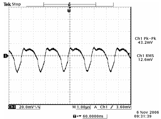
Figure 7. 12 V input, 3.3 V output.
