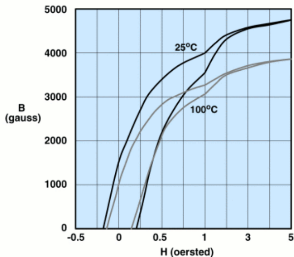
Hysteresis Loop
