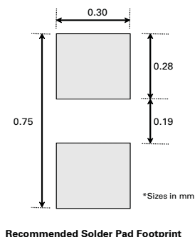
Recommended Solder Pad Footprint
