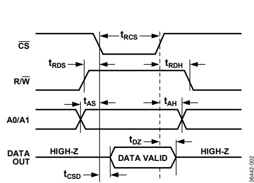
Figure 2. Data Read Timing
