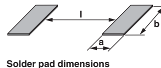
Solder pad dimensions
