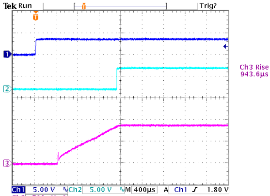
Figure 13: Turn on delay time at 12Vin, 0.9V/60A out (1mS/div) Ch1: Enable, Ch2: PG, Ch3: Vo
