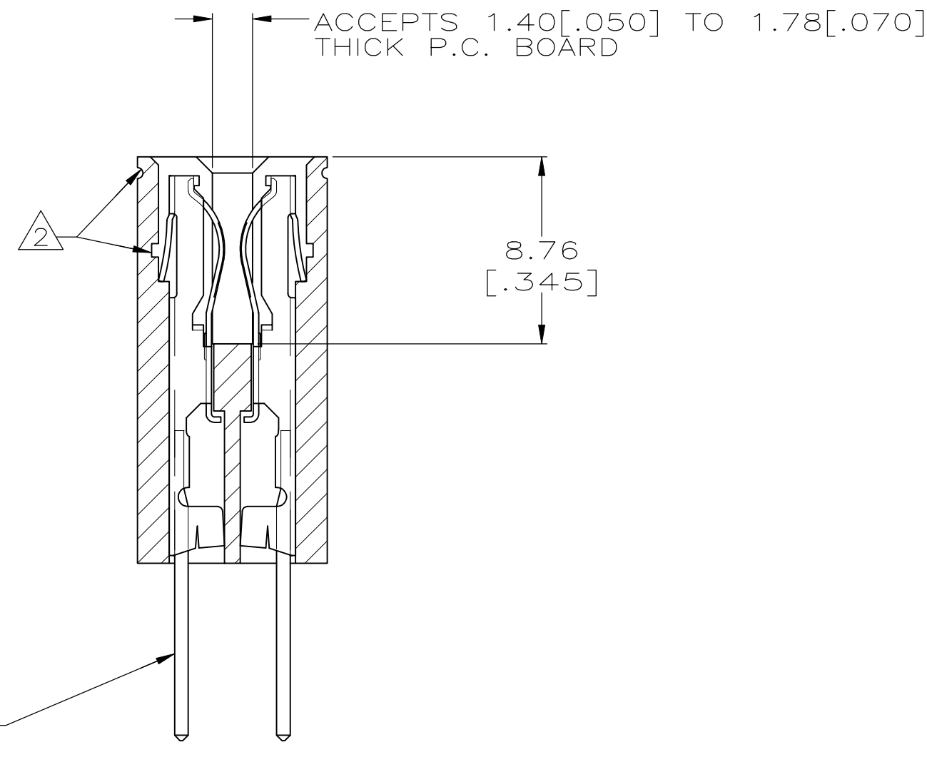
SECTION Z-Z
