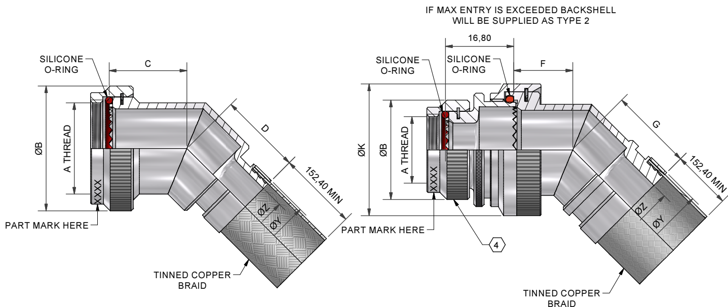
45° BACKSHELL - TYPE 1
