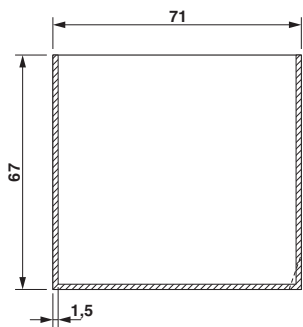
Dimensional drawing
