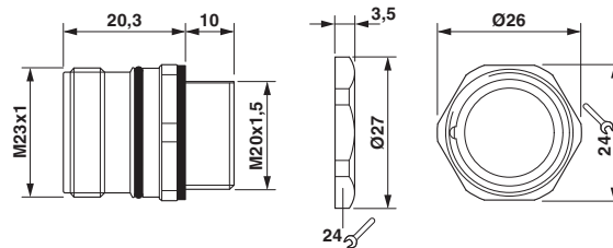
Dimensional drawing
