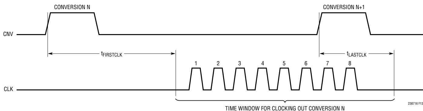
Figure 13. Valid Time Window for Clocking Out Data
