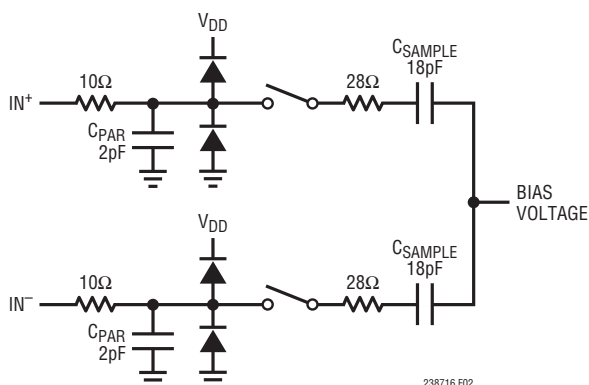
Figure 2. Equivalent Circuit for the Differential Analog Inputs of the LTC2387-16
