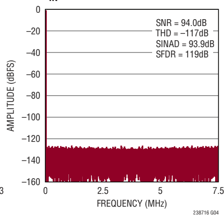
32k Point FFT f_{\text{SAMPL}} = 15\text{Mpsps} , f_{\text{IN}} = 2\text{kHz}
