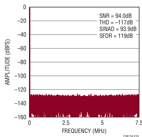
Figure 10. 32k Point FFT of the LTC2387-16, f_{\text{SAMPL}} = 15\text{MSPS} , f_{\text{IN}} = 2\text{kHz}
