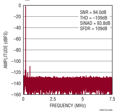
32k Point FFT f_{\text{SAMPL}} = 15\text{Mpsps} , f_{\text{IN}} = 200\text{kHz}
