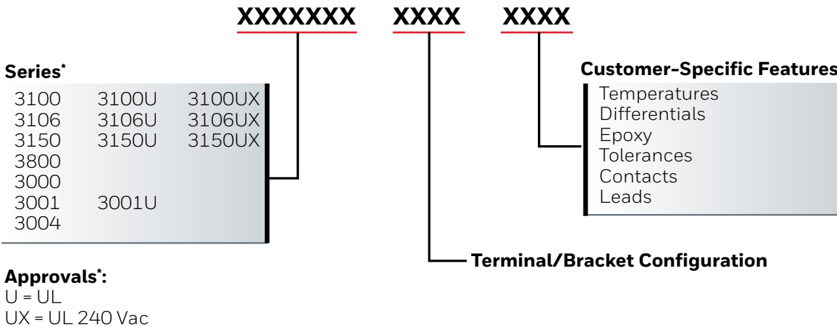
Figure 1. Precision Thermostat Nomenclature
