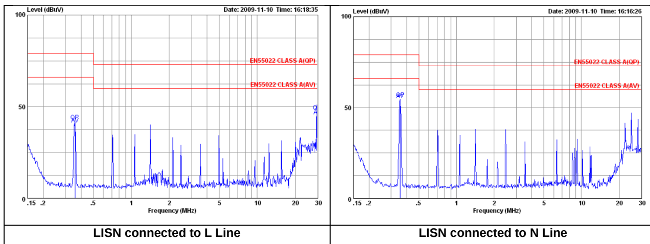
Figure 20. EMC Considerations
