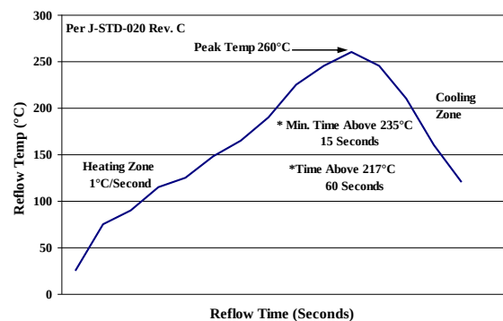
Figure 19. Recommended linear reflow profile using \text{Sn}/\text{Ag}/\text{Cu} solder.
