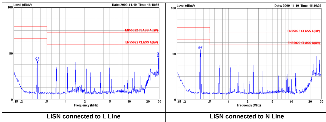
Figure 20. EMC Considerations
