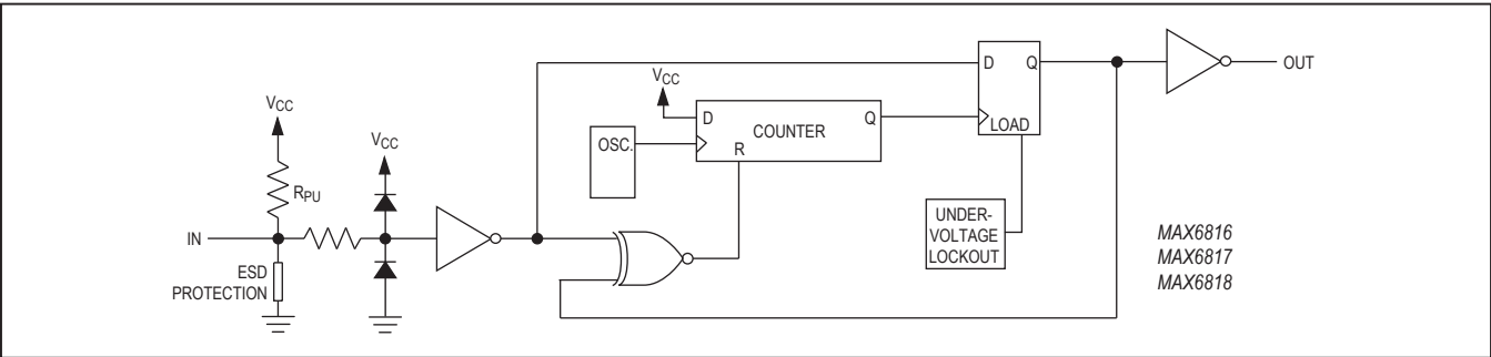
Figure 1. Block Diagram
