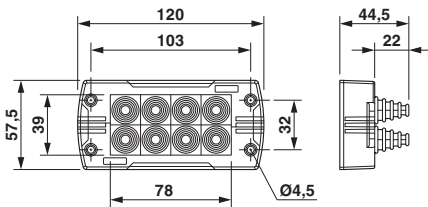
Dimensional drawing
