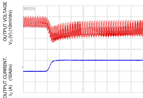
Fig-46. Transient Response to Dynamic Load Change from 50% to 100% at 12Vin, Cout= 1x47uF +11x330uF CTune=47nF, RTune=178 ohms
