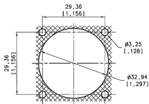
Panel Drilling
