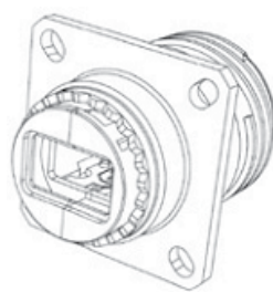
Type 2: Solder 6 Tinned holes for soldering
