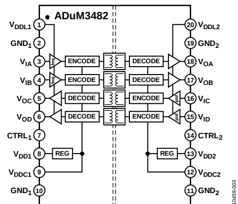
Figure 3. ADuM3482
