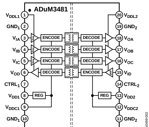
Figure 2. ADuM3481
