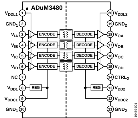
Figure 1. ADuM3480
