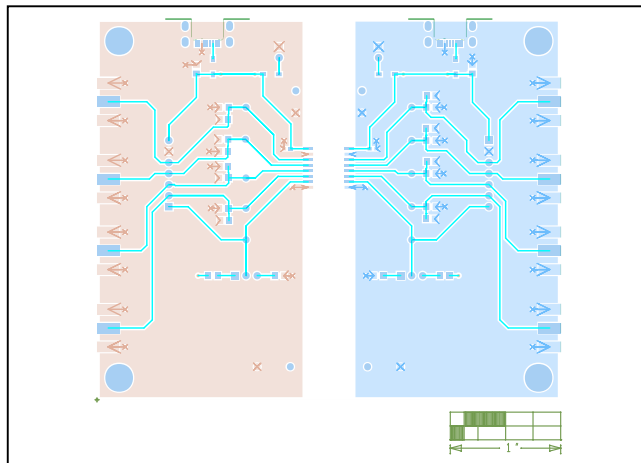
Figure 3. MAX1493X EV Kit PCB Layout (Top Layer)
