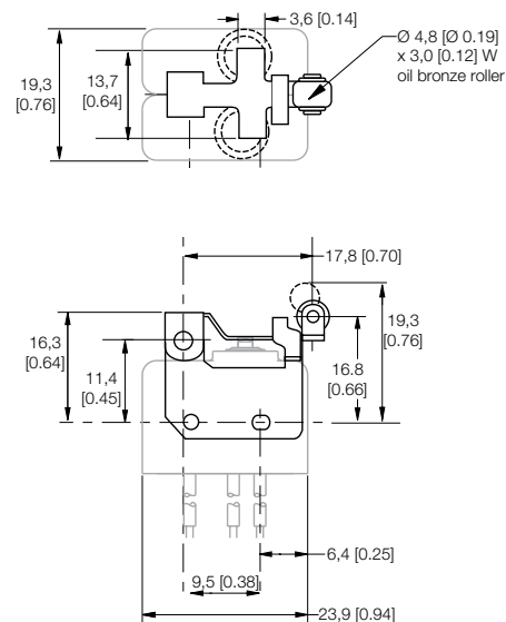
Figure 10. JE-22 Dimensions
