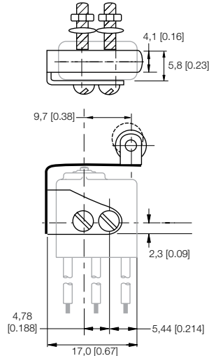
Figure 12. JM-5 Dimensions
