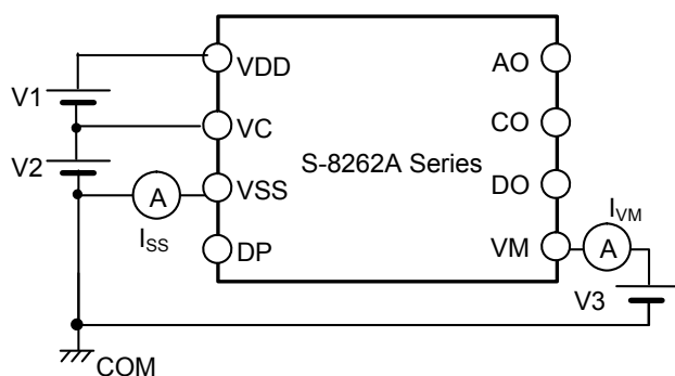
Figure 6 Test Circuit 3
