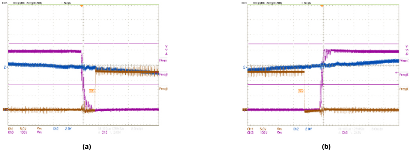
Figure 14. Zero-crossing transitional waveforms (a) from negative to positive half-cycle and (b) from positive to negative half-cycle CH1: V_{GS} gate signal for S_{D2} , CH2: I_L and CH3: V_D
