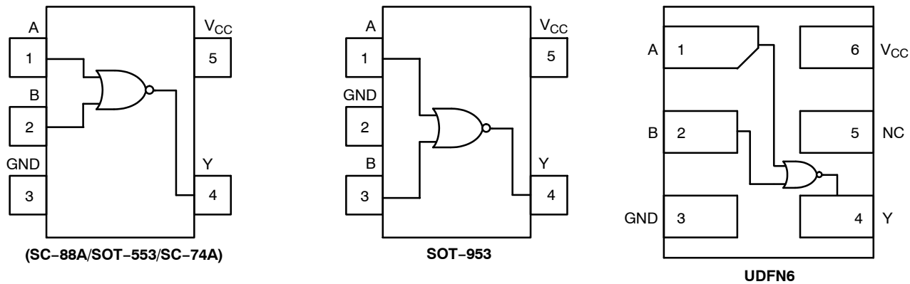
PIN ASSIGNMENT (SC-88A/SOT-553/SC-74A)
