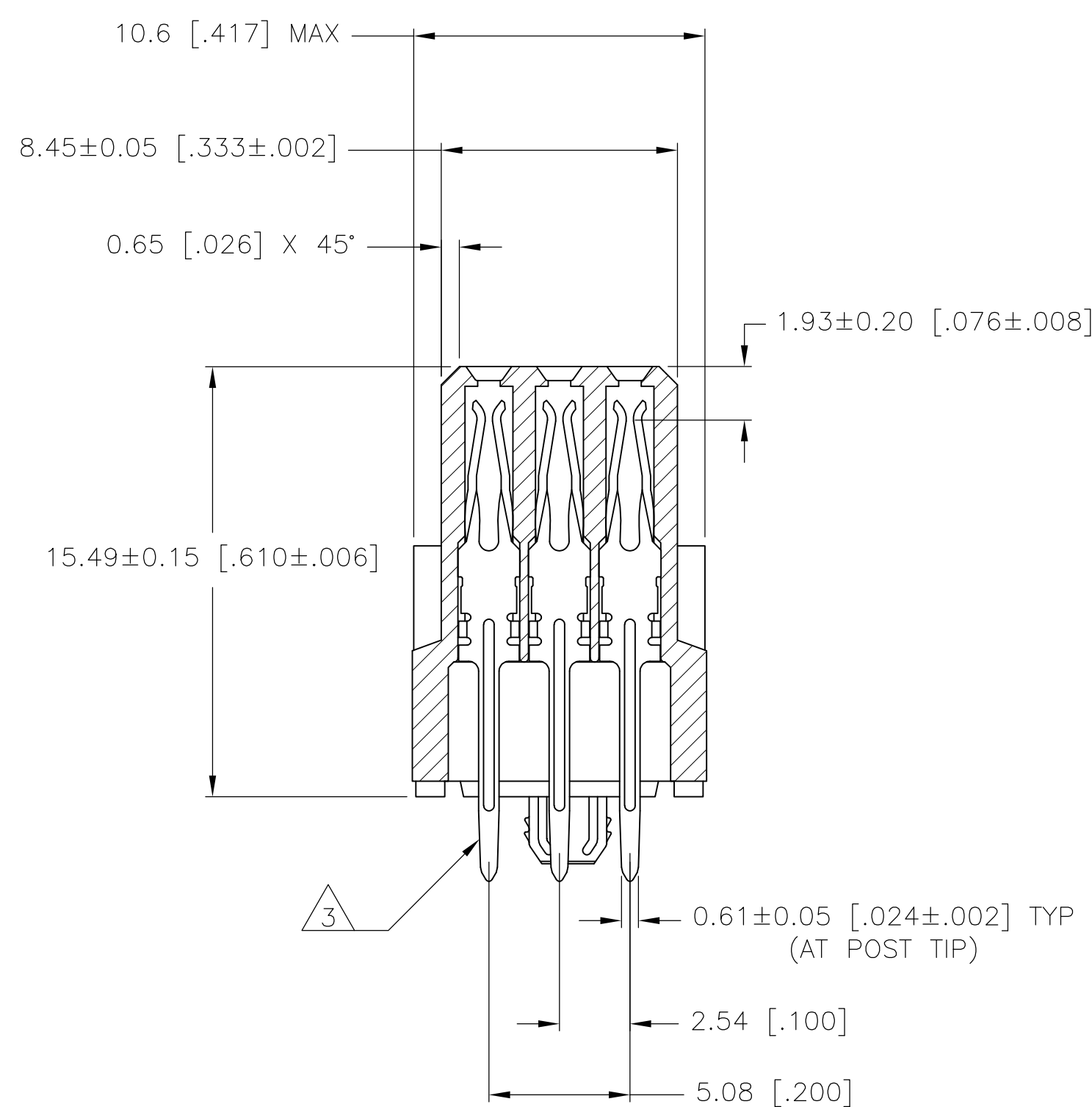
SECTION X-X
