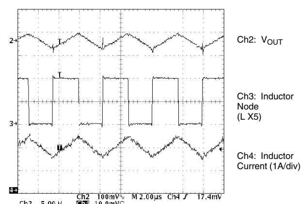
PWM Operation 5 V Converter ( V_{IN} = 10\text{ V} )
