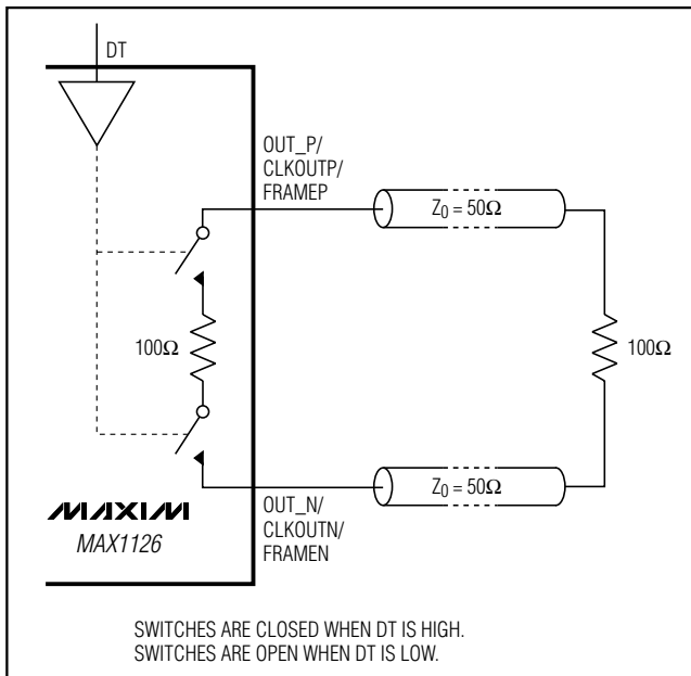
Figure 8. Double Termination
