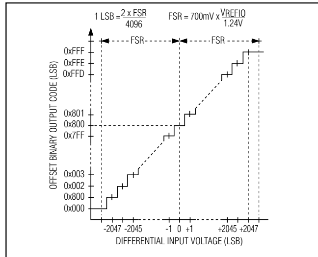
Figure 7. Bipolar Transfer Function with Offset Binary Output Code ( \overline{T}/B = 1 )
