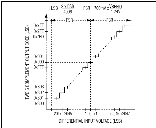
Figure 6. Bipolar Transfer Function with Two's Complement Output Code ( \overline{T}/B = 0 )
