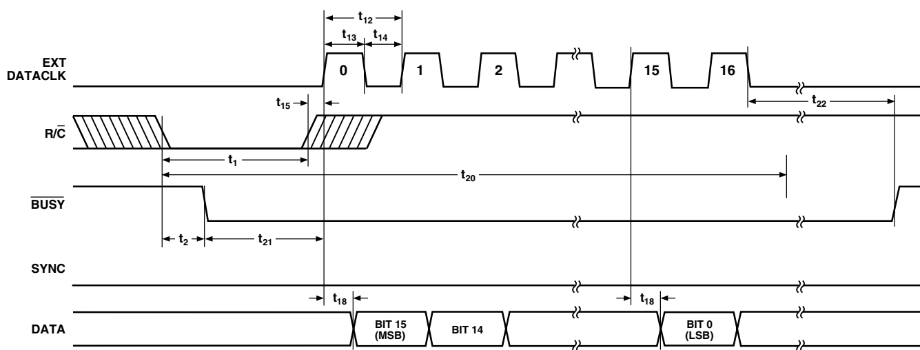
Figure 5. Conversion and Read Timing for Reading Previous Conversion Results During A Conversion Using External Discontinuous Data Clock (EXT/INT Set to Logic High, \overline{CS} Set to Logic Low)
