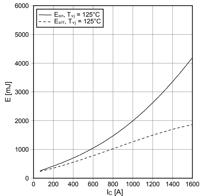
Schaltverluste IGBT-Wechselr. (typisch) switching losses IGBT-inverter (typical) E_{on} = f(I_c), E_{off} = f(I_c) V_{GE} = \pm 15\text{ V}, R_{Gon} = 1.4\ \Omega, R_{Goff} = 1.8\ \Omega, V_{CE} = 1800\text{ V}, C_{GE} = 150\text{ nF}
