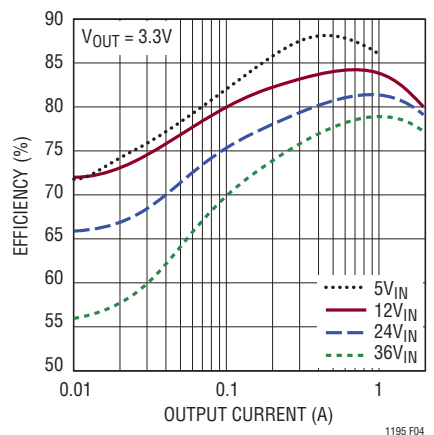
Figure 4. Efficiency
