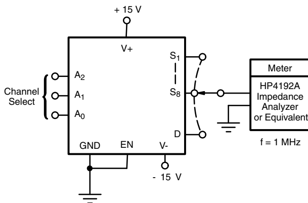
Fig. 9 - Source Drain Capacitance
