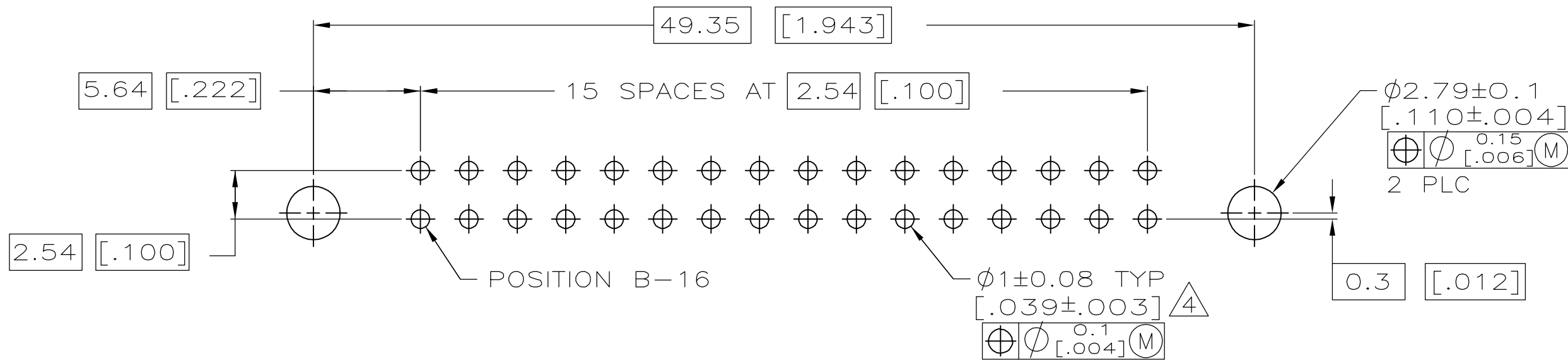
PC BOARD LAYOUT
