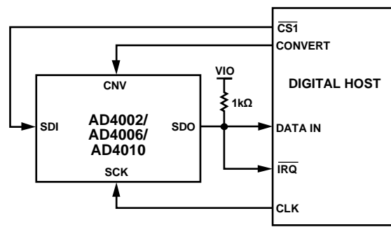
Figure 57. \overline{CS} Mode, 4-Wire Turbo Mode Connection Diagram
