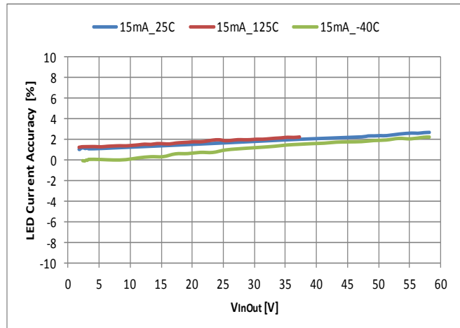
Figure 13 LED Current Accuracy (%) vs. V INOUT Across Temperature
