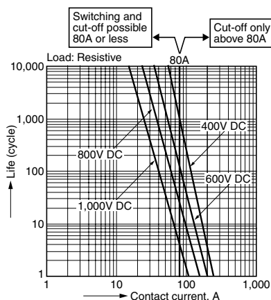
3.-(3) Switching life and cut-off curves (80A type)
