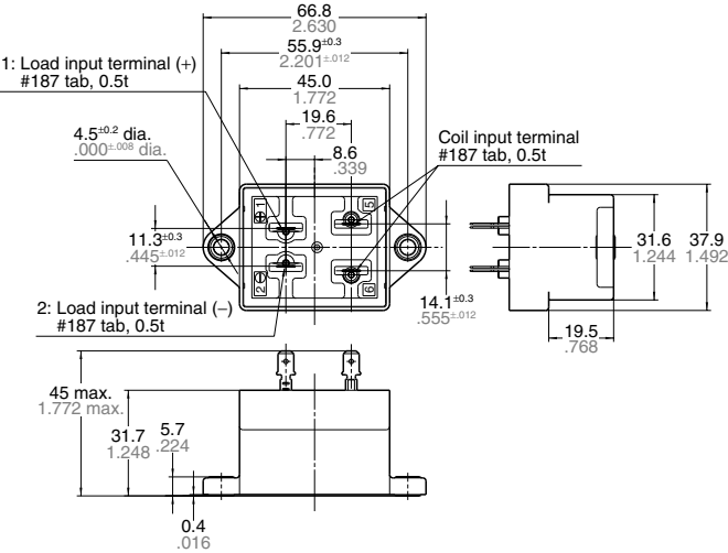
External dimensions
