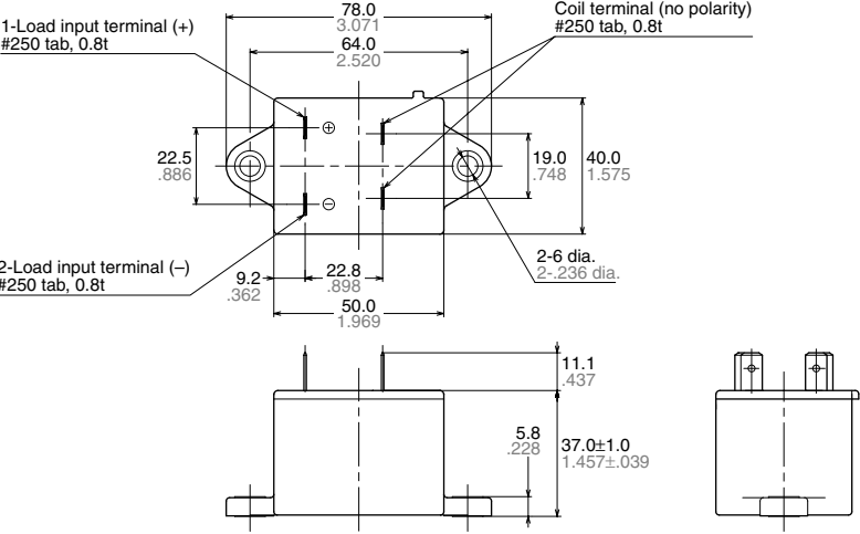
External dimensions
