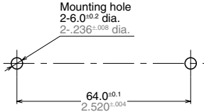
Panel cut-off
